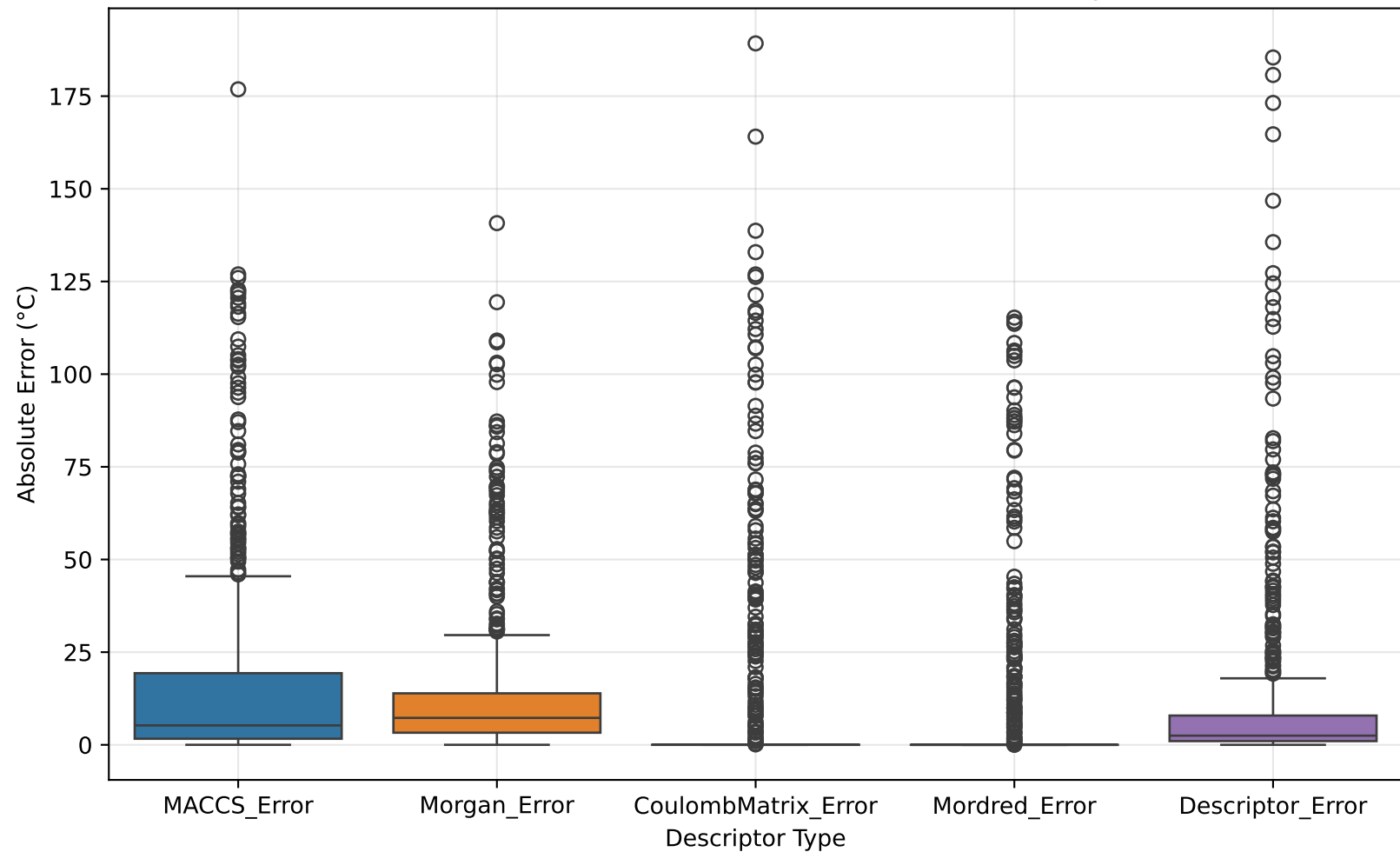
Absolute Error Distributions of XGBoost Across Descriptors
